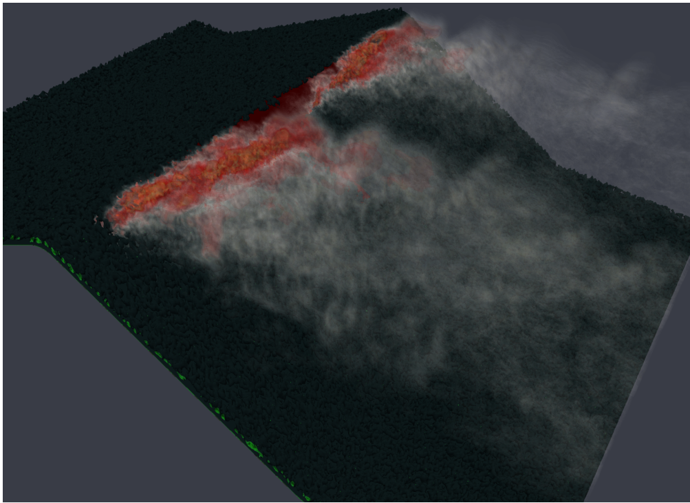
Figure 5: Back curve fire on a mountain topography
