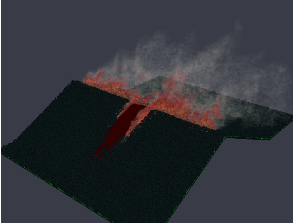
Figure 4: Head curve fire on a mountain topography
