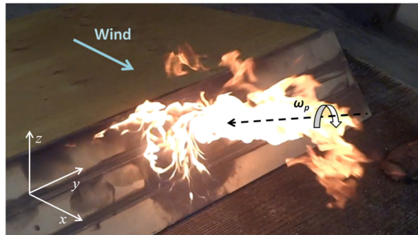
Figure 3: Experimental fire in a wind tunnel showing a fire vortex on the leeward slope of an idealized ridge. Figure credit Sharples et al. [4]
