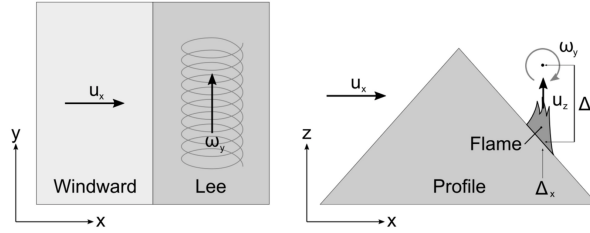
Figure 2: A diagram of vorticity-driven lateral spread. Figure credit Sharples et al. [4]
