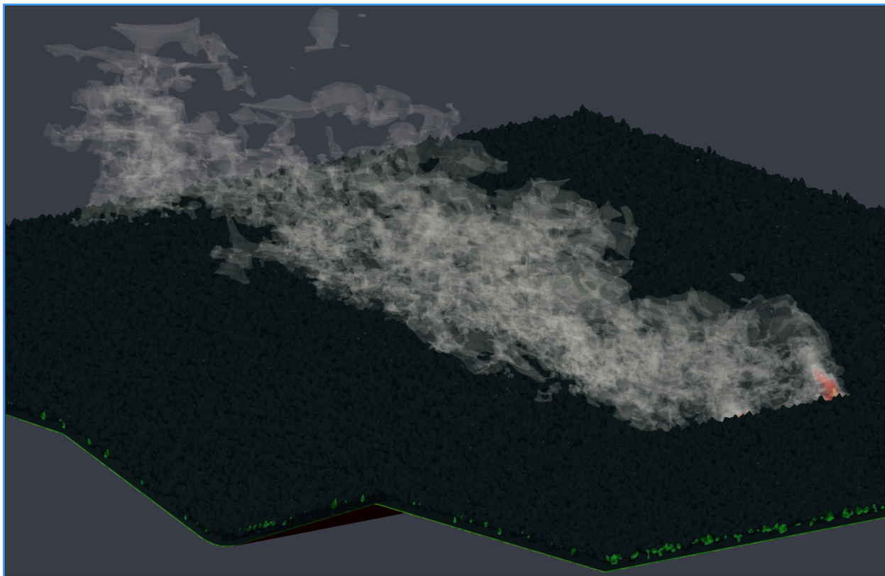
Figure 1: A valley wildfire modeled using topography from the Los Alamos Los Conchas Fire.
